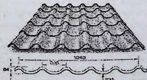
Metallocherepitsa listi
