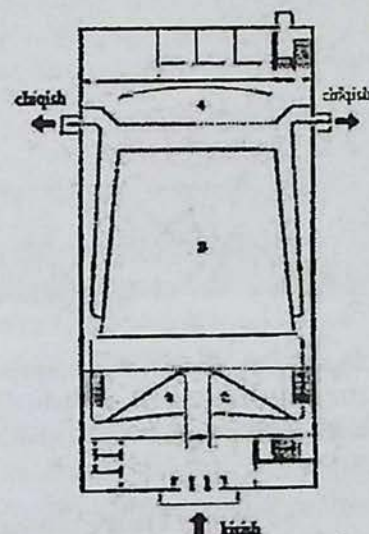
Kinoteatr. Rejalashtirishning zalli tizimi:
