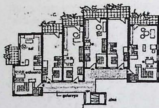
Galereyali uy qavatining rejalari
