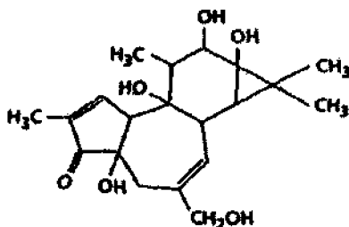
Forbol
