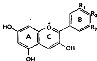
Antostionidin
