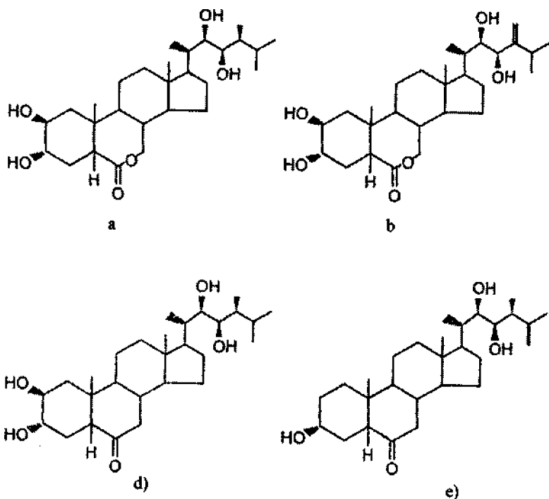
II.11-rasm. Brassinsteroidlar:
