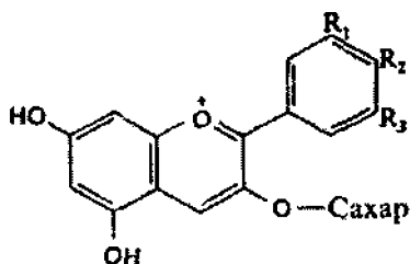
Antostionidinni tuzilishi
