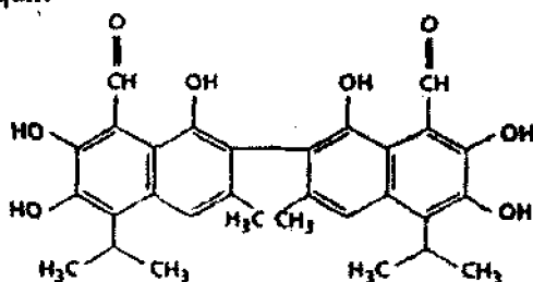
Gossipol
