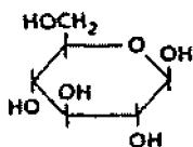
\beta -D-glyukoza
