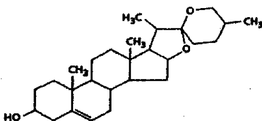
Yamogenin
