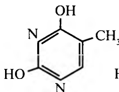
timin
