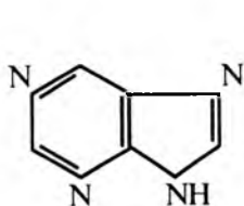
purin
