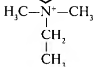
Endofonyl
