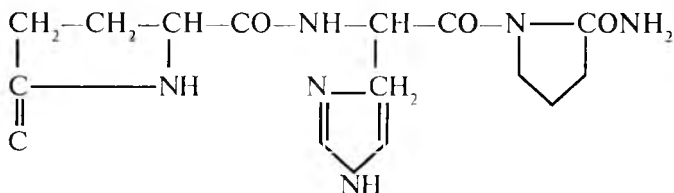
Piroglutamil-gistidil-prolinamid
