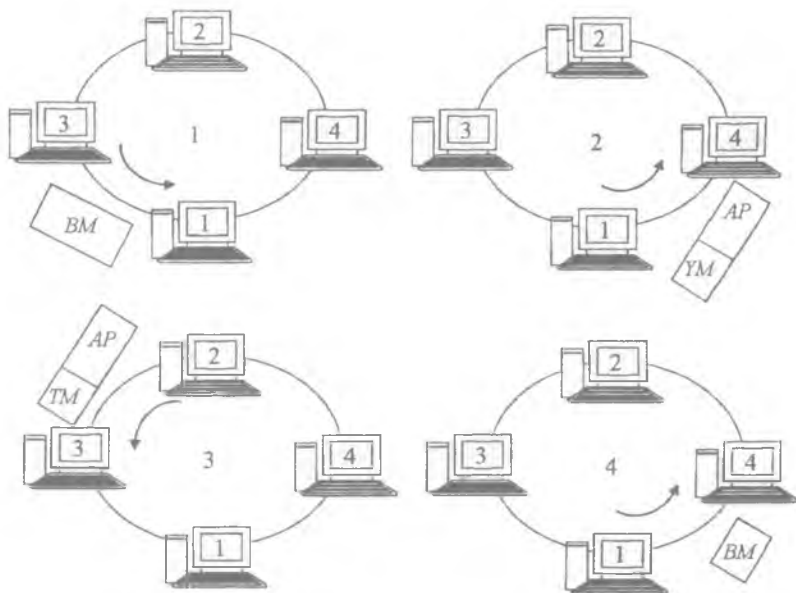
5.22-rasm. Almashinuvni marker usuli yordamida boshqarish (BM–bo‘sh marker, YUM–yuklangan marker, TM – bandligi tasdiqlangan marker, AP – axborotlar paketi).
