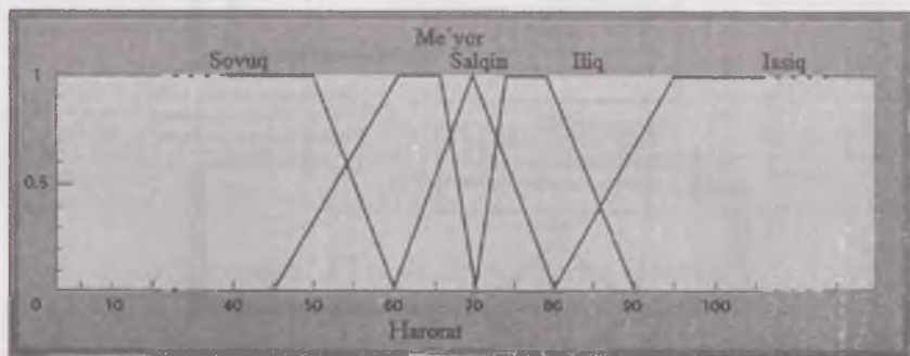
3.9.8-rasm. Haroratni o'lchash mantig'i
