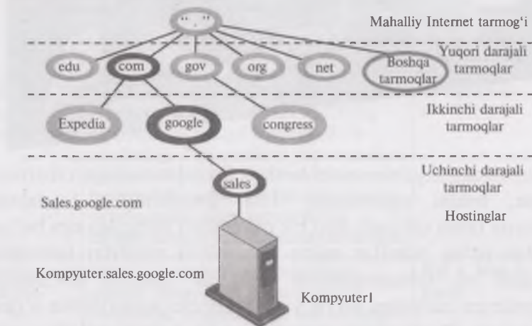
2.4.3-rasm. Domen nomlanish tizimi
