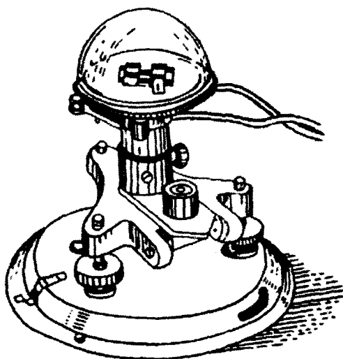
18-rasm. Piranometrning tashqi ko'rinishi.
