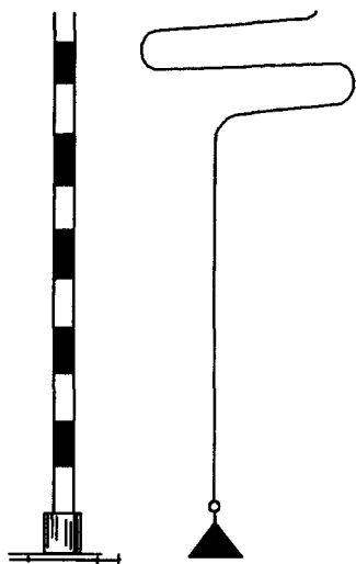
25-rasm. Suvning chuqurligini o'lchagich.
