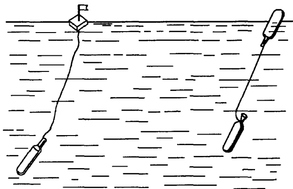
26-rasm. Suv oqimining tezligini o'lchaydigan moslama.
