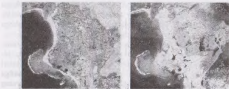
23.1-rasm. Landshaftlarning o'zgarishi: Tailanddagi sunamidan oldin va keyin 2
