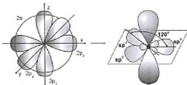
3- rasm. Uglerod atomining sp^2 - gibridlanishi.
