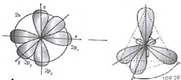
1- rasm. Uglerod atomining sp 3 - gibridlanishi.
