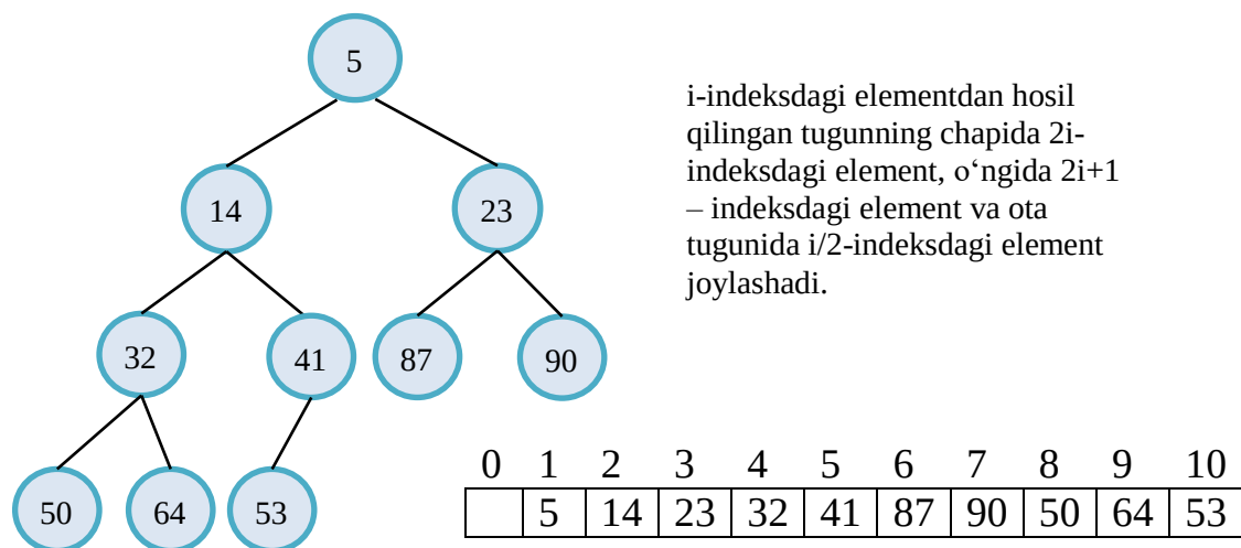
4.11-rasm. Heap tree tuzilmasini tuzish
