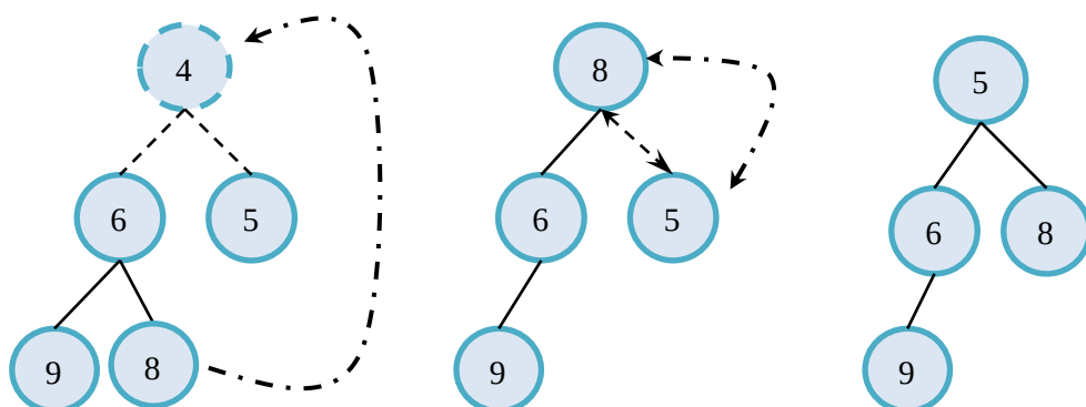
4.15-rasm. Min-heap tuzilmasidan elementni o‘chirish amali
