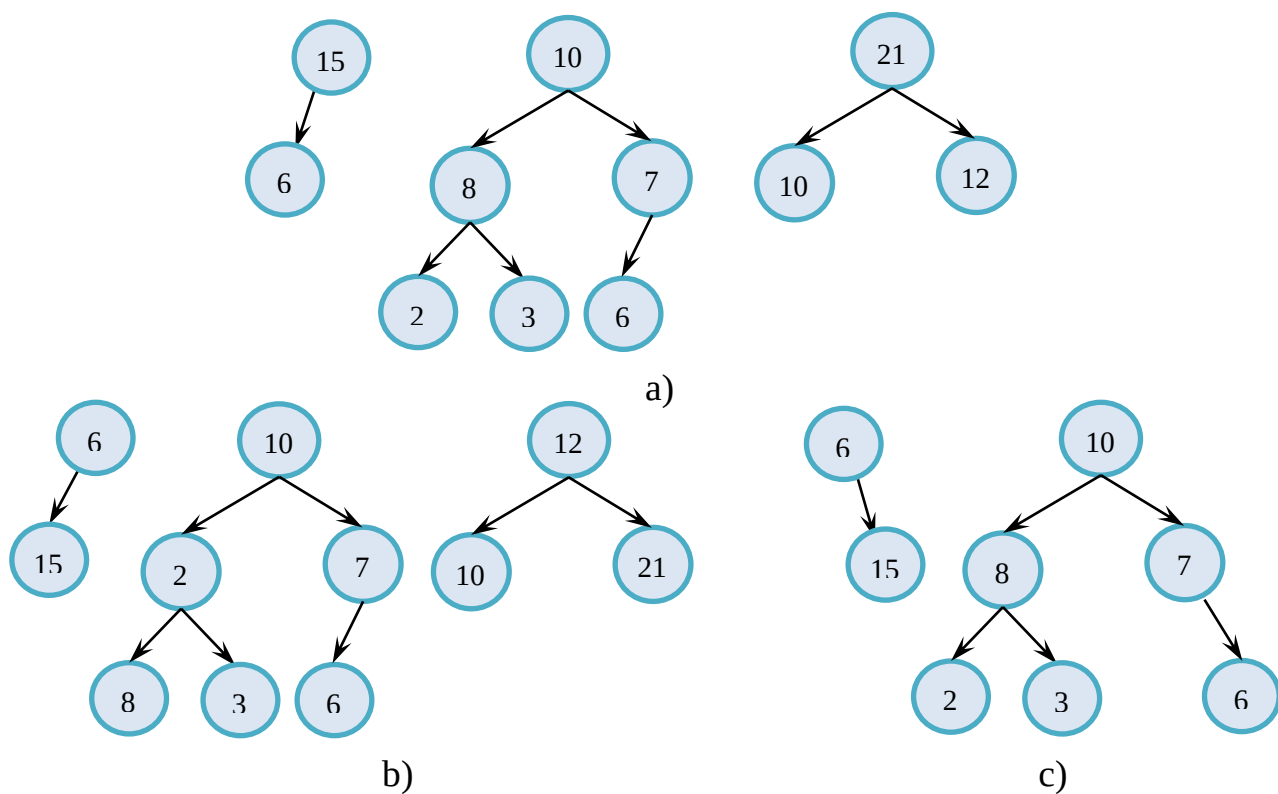
4.9-rasm. Heap tree (a) va heap tree bo'lmagan daraxtlar
