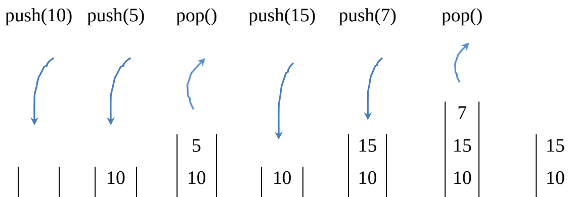
3.5 – rasm. Stekda bajarilgan amallar ketma – ketligi
