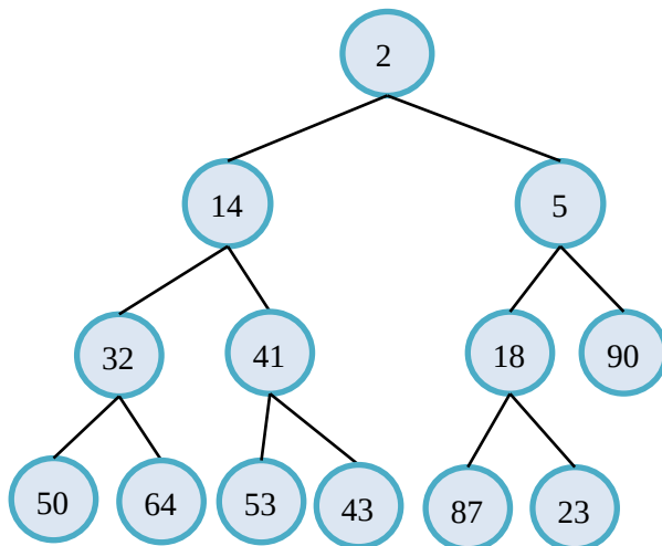
4.14-rasm. Min-heap tuzilmasiga yangi element kiritish
