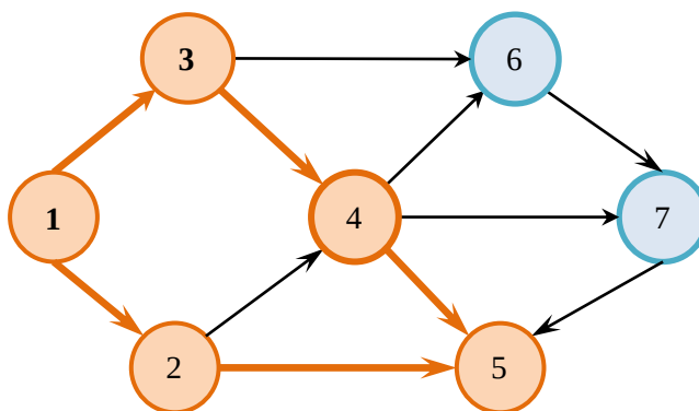
4.26-rasm. Grafdagi halqa
