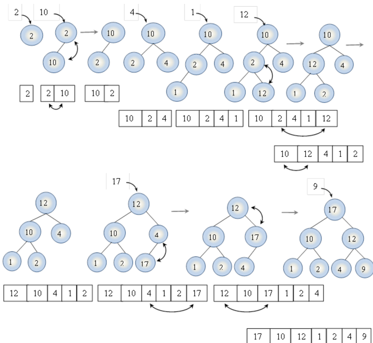
4.16-rasm. Max-heap tree tuzilmasini "yuqoridan-pastga" usuli bilan tashkil etish
