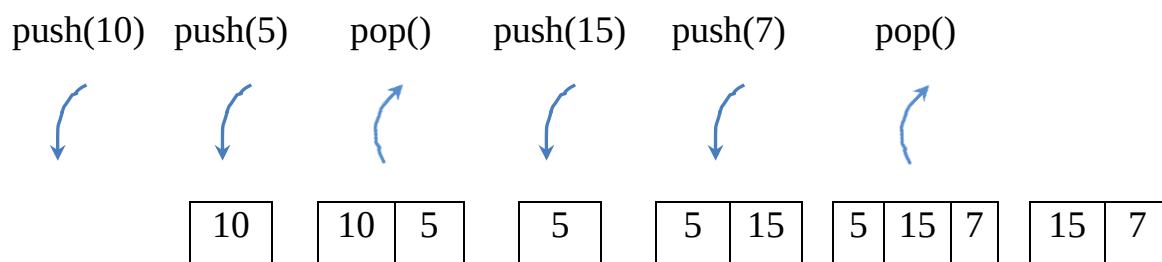
3.7-rasm. Navbatda ketma – ket amallar bajarish
