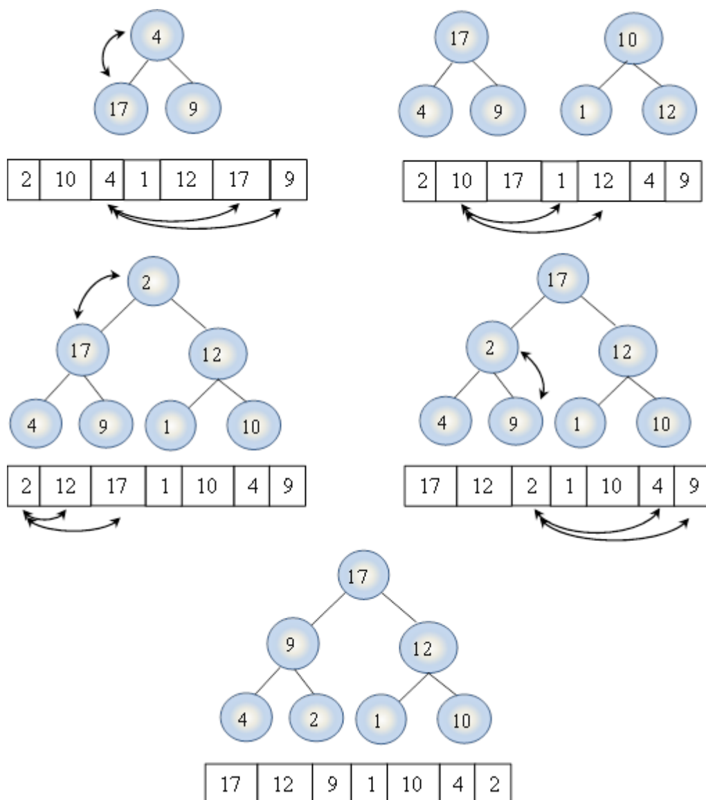
4.17-rasm. Arr[2, 10, 4, 1, 12, 17, 9] massivni “pastdan-yuqoriga” usuli bilan
