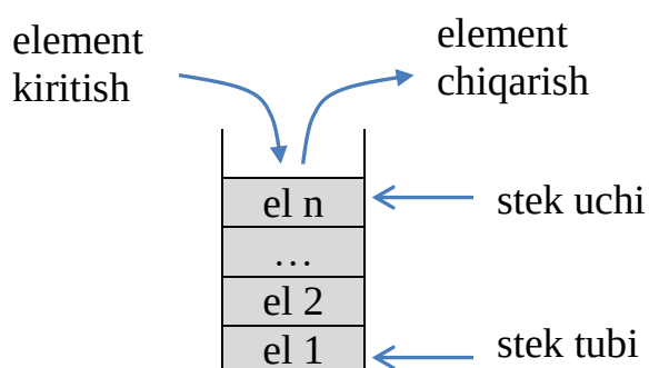
3.4-rasm. Stek tuzilishi
