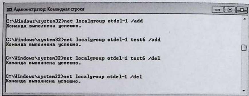
3.32-rasm. Yangi guruh yaratish (o'chirish), net localgroup buyrug'i yordamida foydalanuvchini guruhga qo'shish (o'chirish)
