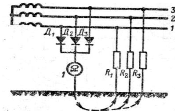
40- rasm. Uch ventel sxemasi
