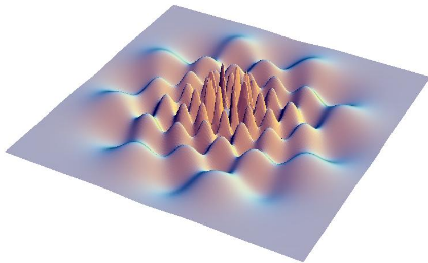
c / A cross-section of a hydrogen wavefunction.
