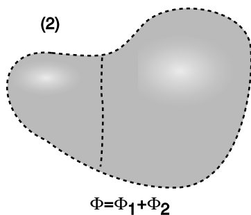
e / 1. The flux due to two charges equals the sum of the fluxes from each one. 2. When two regions are joined together, the flux through the new region equals the sum of the fluxes through the two parts.
