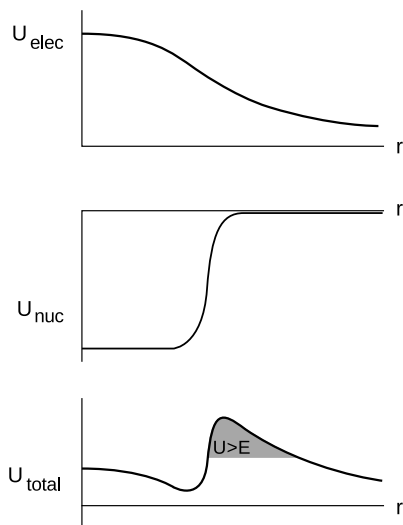
n / The electrical, nuclear, and total interaction energies for an alpha particle escaping from a nucleus.
