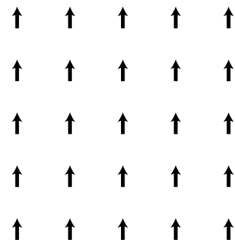
d / The field \hat{y} .
