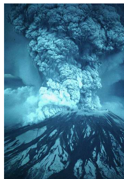
a / In 1980, the continental U.S. got its first taste of active volcanism in recent memory with the eruption of Mount St. Helens.
