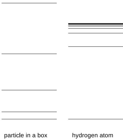
f / The energy levels of a particle in a box, contrasted with those of the hydrogen atom.
