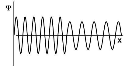
o / A particle encounters a step of height U < E in the interaction energy. Both sides are classically allowed. A reflected wave exists, but is not shown in the figure.
