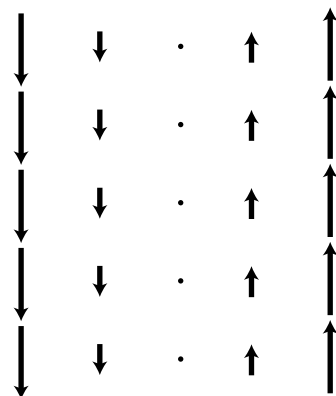
e / The field x\hat{y} .
