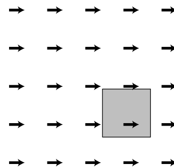
c / The field \hat{x} .
