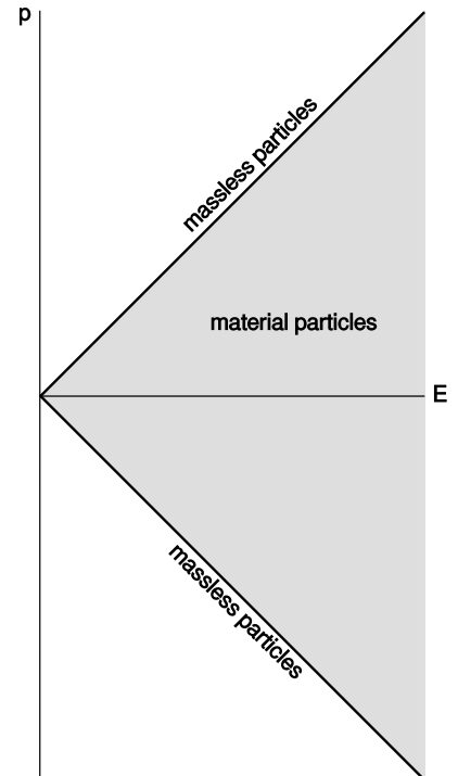
g / In the p - E plane, massless particles lie on the two diagonals, while particles with mass lie to the right.
