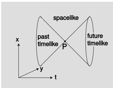
aa / The light cone.
