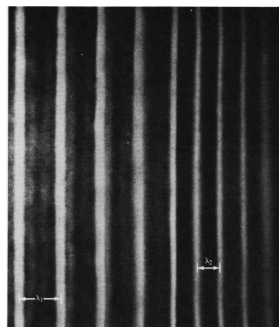
u / A water wave traveling into a region with different depth will change its wavelength.
