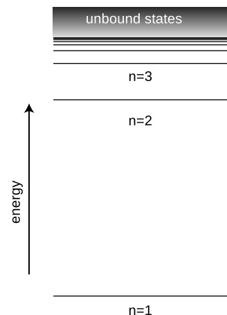
d / The energy of a state in the hydrogen atom depends only on its n quantum number.
