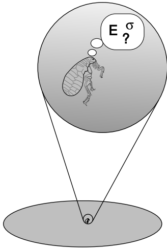
h / Close to the surface, the relationship between E and \sigma is a fixed one, regardless of the geometry. The flea can't determine the size or shape of her world by comparing E and \sigma .
