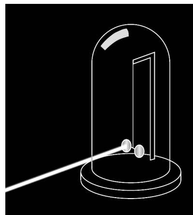
q/A simplified drawing of the 1903 experiment by Nichols and Hull that verified the predicted momentum of light waves. Two circular mirrors were hung from a fine quartz fiber, inside an evacuated bell jar. A 150 mW beam of light was shone on one of the mirrors for 6 s, producing a tiny rotation, which was measurable by an optical lever (not shown). The force was within 0.6% of the theoretically predicted value (problem 11 on p. 441) of 0.001 \mu\text{N} . For comparison, a short clipping of a single human hair weighs \sim 1 \mu\text{N} .
