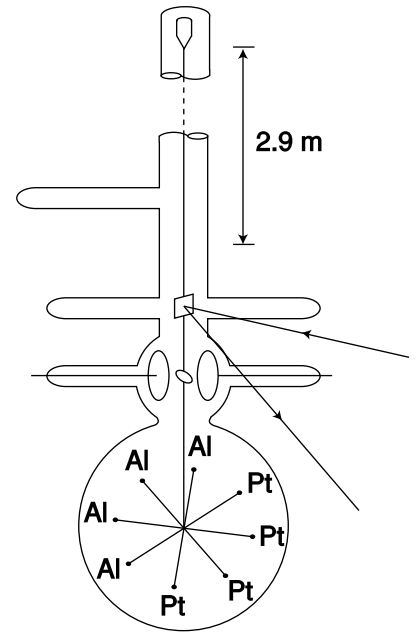
d / A more realistic drawing of Braginskii and Panov's experiment. The whole thing was encased in a tall vacuum tube, which was placed in a sealed basement whose temperature was controlled to within 0.02^\circ\text{C} . The total mass of the platinum and aluminum test masses, plus the tungsten wire and the balance arms, was only 4.4 g. To detect tiny motions, a laser beam was bounced off of a mirror attached to the wire. There was so little friction that the balance would have taken on the order of several years to calm down completely after being put in place; to stop these vibrations, static electrical forces were applied through the two circular plates to provide very gentle twists on the ellipsoidal mass between them. After Braginskii and Panov.
