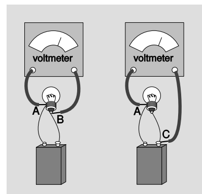
i / The voltmeter doesn't care which of these setups you use.
