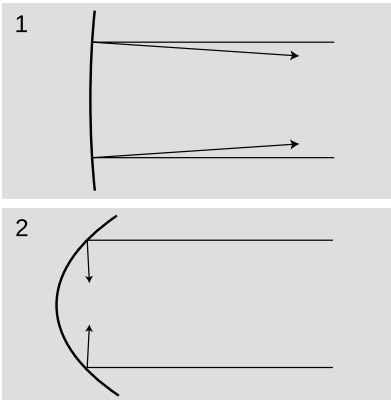
e/Mirror 1 is weaker than mirror 2. It has a shallower curvature, a longer focal length, and a smaller focal angle. It reflects rays at angles not much different than those that would be produced with a flat mirror.
