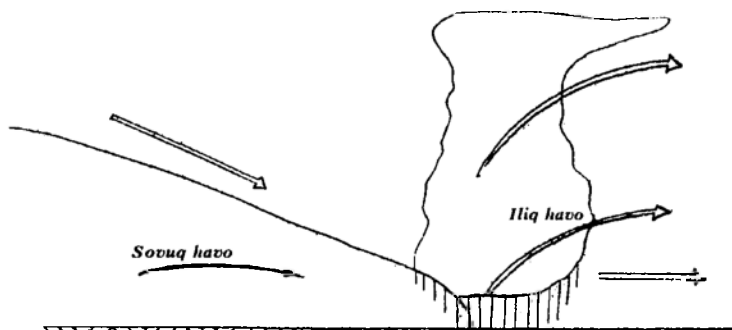
34-rasm. Sovuq front.
